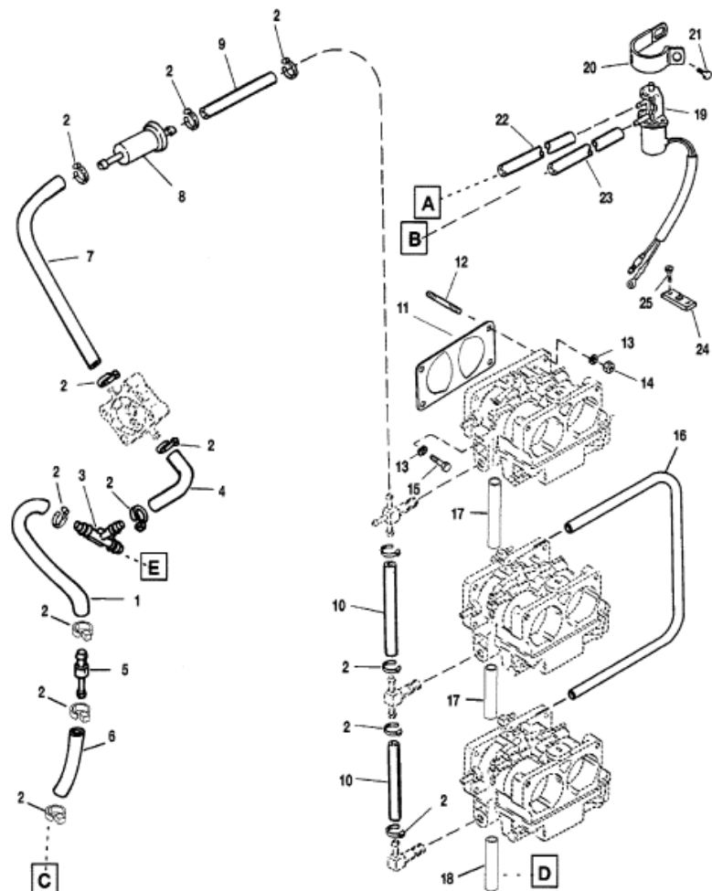
A= to top carb . . B = to middle carb . . . . C = to oil pump . D= to Cyl. Head . E = to primer bulb
